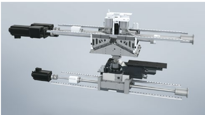
Delta Drive: This innovative drive concept offers novel processing and discharging options.
